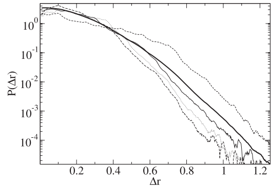
Figure 4. P(\Delta r) for several consecutive intervals with \Delta\gamma = .002 . The average over all intervals from \gamma = 12\% to 24\% is shown in heavy black.
