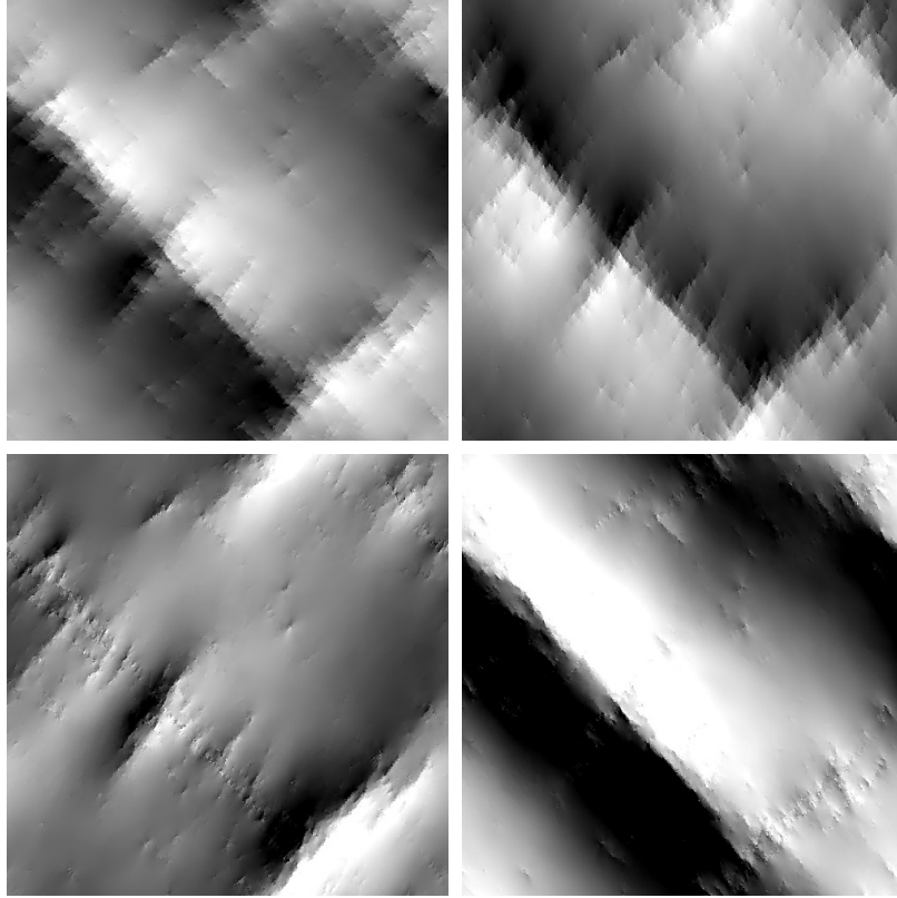
Figure 1. Grayscale plots of the projections of a typical non-affine displacement field \Delta\vec{r} onto different directions. Top left: \Delta x . Top right: \Delta y . Bottom left: (\Delta x + \Delta y)/\sqrt{2} . Bottom right: (\Delta x - \Delta y)/\sqrt{2} . Here \Delta\gamma = 0.002 , the x -axis is horizontal, and the gray scale is linear, ranging from -\sigma_0 (black) to +\sigma_0 (white).
