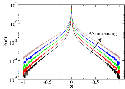
Figure 7. The time averaged \omega distributions, P(\omega; \Delta\gamma) for \Delta\gamma = 0.001, 0.002, 0.004, 0.008, 0.016 .
