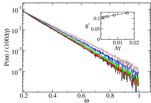
Figure 8. Distribution of \omega scaled by \Delta\gamma in per cent for \Delta\gamma = 0.001, 0.002, 0.004, 0.008, 0.016 . Curves increase with \Delta\gamma at large \omega . Straight lines show exponential fits, P \propto e^{-\omega/\omega^*} , and the inset shows \omega^* as a function of \Delta\gamma . Curves for higher \Delta\gamma are higher as in figure 7.
