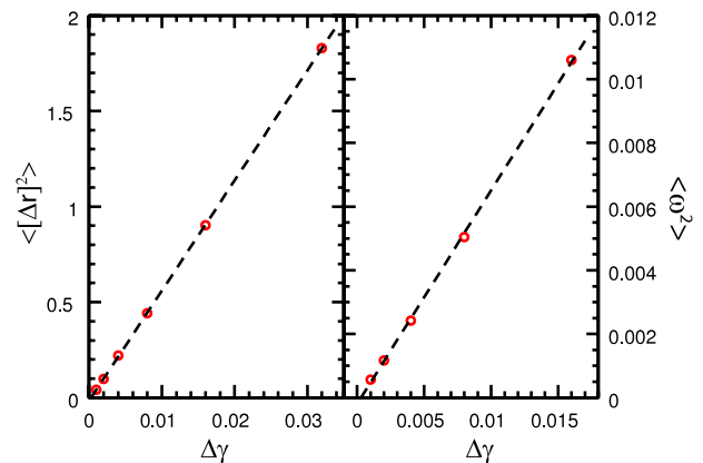
Figure 5. Variation with \Delta\gamma of the mean-squared (left) displacement \langle \Delta r^2 \rangle and (right) strain \langle \omega^2 \rangle . Straight lines are linear fits through the data points, which have statistical errors that are slightly smaller than the symbol size.
