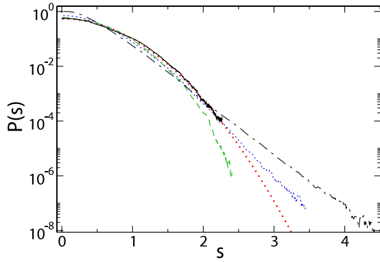
Figure 6. Average displacement distributions, P(\Delta r; \Delta\gamma) , for \Delta\gamma = 0.001 (dot-dashed), 0.002 (dotted), 0.008 (dashed), and 0.032 (solid). To compensate for the increase in width with \Delta\gamma , the curves are plotted as a function of s \equiv \Delta r/\sigma_0(100\Delta\gamma)^{0.5} . The thick (red) dotted line is a one-parameter fit of the \Delta\gamma = 0.032 data to a Gaussian. Averages are over all intervals from \gamma = 12\% to \gamma = 24\% .
