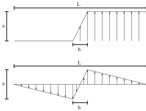
Figure 2. An idealized schematic representation of the (top) total and (bottom) non-affine displacements parallel to a slip line as a function of distance away from the line. The change a in the total displacement across the periodic cell is accommodated in a plastic zone of width h where the displacement changes rapidly, \omega \approx a/h . The total displacement in the surrounding elastic regions is nearly constant. Subtracting the affine displacement associated with a strain \Delta\gamma leads to a small gradient, \omega \approx \Delta\gamma , in the elastic regions of plots of the non-affine displacement.
