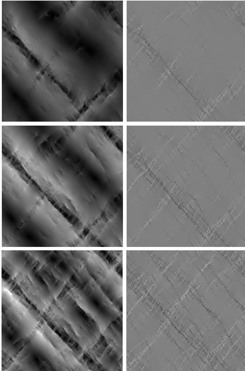
Figure 3. Left: the magnitude, \Delta r , of the (non-affine) displacement fields. Gray scale is linear ranging from 0 (black) to +2.5\sigma_0 (white). Right: the curl, \omega , of the (non-affine) displacement fields. Gray scale is linear ranging from -0.25 (black) to +0.25 (white). Displacements are computed relative to the same initial state as in figure 1 and over growing strain intervals \Delta\gamma = 0.002 (top), 0.004 (center), and 0.008 (bottom).
